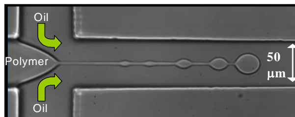
Figure 1: Polymer fluid filament being stretched by an immiscible oil fluid of same shear viscosity in a 50 \mu\text{m} cross-slot microchannel.
